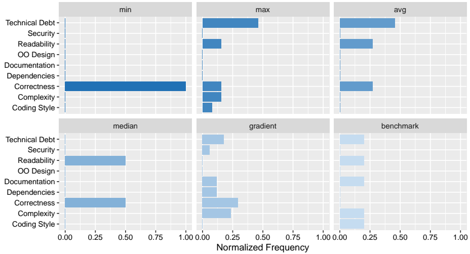
Fig. 6: Usage Patterns of Time Series Operations.
